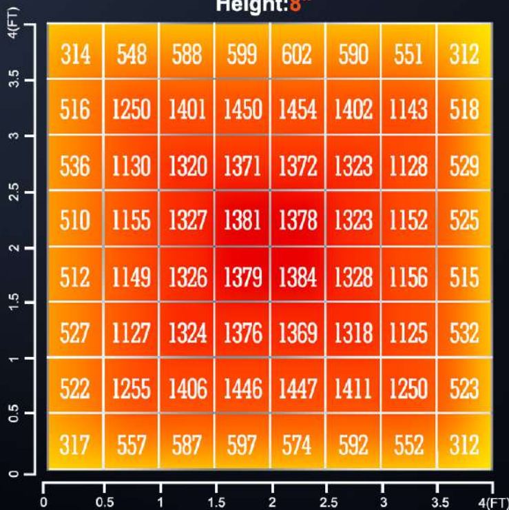
Height: 8"
