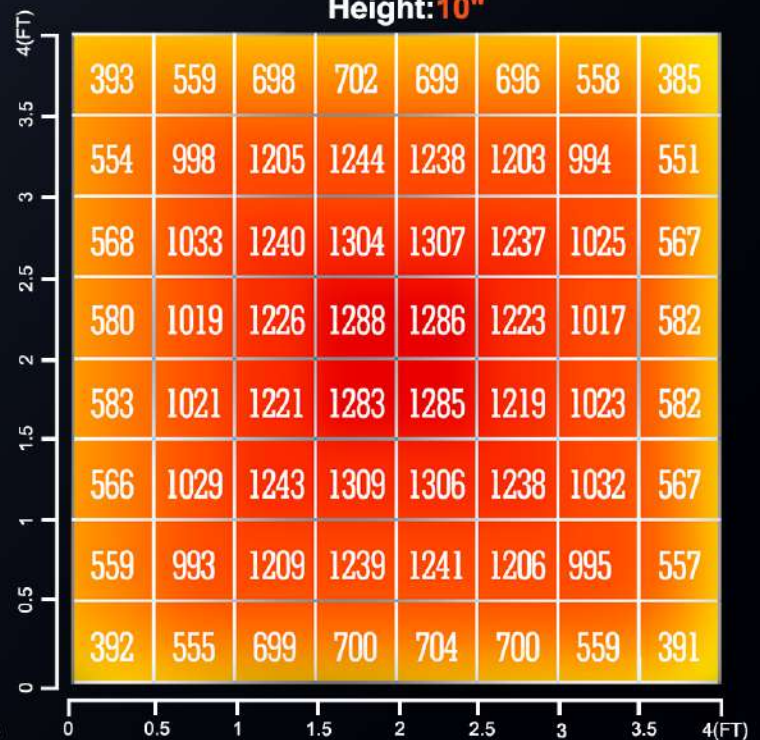
Height: 10"
